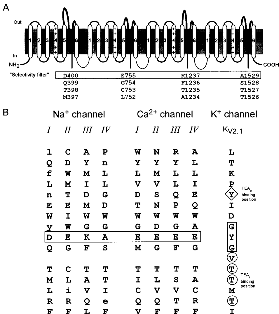
FIGURE 1 (A) Transmembrane topology of the \text{Na}^+ channel. The P segments are the regions between the fifth and sixth membrane-spanning repeats in each domain ( bold line ). The approximate position of the residues that were mutated are enclosed in the box and shown below the topology cartoon. The putative selectivity residues D400, E755, K1237, and A1529 are shown for reference. (B) Single-letter amino acid alignment of the residues in the P segments of the rat skeletal muscle \mu 1 \text{Na}^+ channel (Trimmer et al., 1989) are anchored by the DEKA selectivity filter ( enclosed in the box ). The uppercase letters in the \text{Na}^+ and \text{Ca}^{2+} channel sequences signify conservation of the residue across all channel isoforms. The \text{Na}^+ channel P segments show sequence homology to the \text{Ca}^{2+} channel (Tanabe et al., 1987), but little to the \text{K}^+ channel (Frech et al., 1989). The residues enclosed in the rectangle are the \text{K}^+ channel signature sequence; those enclosed in circles are accessible to MTSET from the intracellular side of the channel (Pascual et al., 1995), and the tyrosine (Y) inside the diamond and the threonine (T) in the circle are the extracellular and intracellular TEA binding sites, respectively (MacKinnon and Yellen, 1990).
