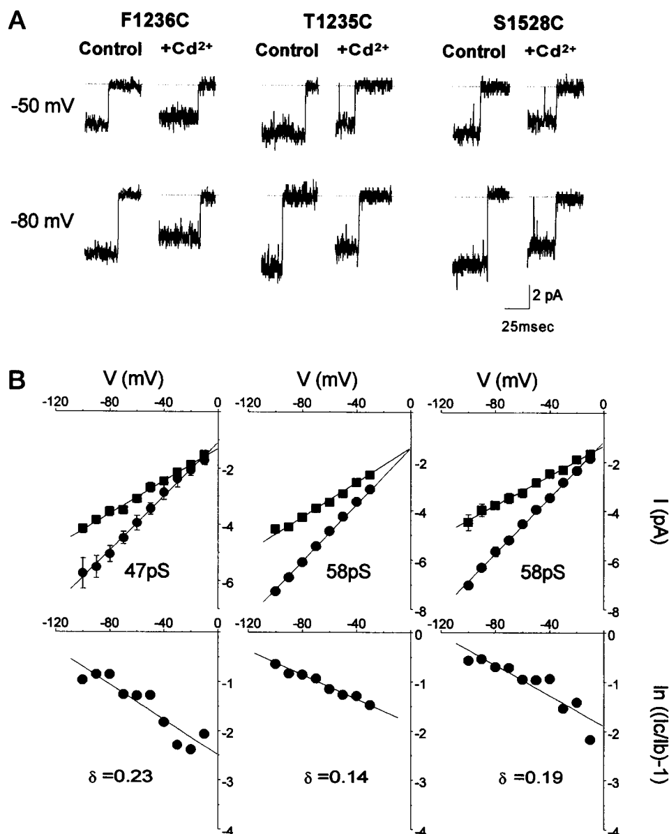
FIGURE 7 Single-channel \text{Cd}^{2+} block of cysteine mutants. (A) Representative single-channel currents after modification by 20 \mu\text{M} fenvalerate, elicited by voltage steps to -50 and -80 mV with 140 mM \text{Na}^+ in the pipette. The single-channel current is reduced in the presence of 500 \mu\text{M} (F1236C and T1235C) and 800 \mu\text{M} (S1528C) \text{Cd}^{2+} . (B) Single-channel current-voltage relationships for each of the mutant channels determined from at least three patches in the absence of \text{Cd}^{2+} , the slope conductances are within 20% of that of the wild-type channel ( top ). \text{Cd}^{2+} blocks each of the mutants in a voltage-dependent fashion. A plot of the logarithm of the ratio of the blocked and unblocked single-channel current amplitude versus voltage gives the fractional electrical distance ( \delta ) for \text{Cd}^{2+} binding ( bottom ).
