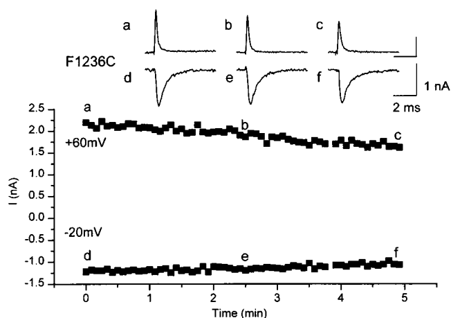
FIGURE 3 Internal MTSEA does not modify the current through the P segment mutants. The time course of the peak current through the F1236C mutant elicited by voltage steps from -100 mV to -20 and +60 mV after establishment of the whole-cell patch configuration (time 0) with 1 mM MTSEA in the pipette. The currents labeled a–f were acquired at the time of break-in (a, d) and at 2.5 (b, e) and 5 (c, f) min of cell dialysis. There is no change in the current amplitude after cell dialysis; the small reduction observed at the +60 mV test potential is the result of rundown.
