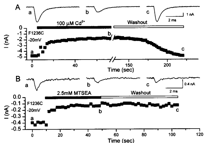
FIGURE 5 Effects of external \text{Cd}^{2+} and MTSEA on F1236C. (A) The current through F1236C is reversibly inhibited by 100 \mu M \text{Cd}^{2+} in the bath solution. Current records elicited by voltage steps from -100 to -20 mV before ( a ), during ( b ), and after ( c ) perfusion with 100 \mu M \text{Cd}^{2+} . (B) Time course of inhibition of F1236C current by bath application of 2.5 mM MTSEA. The current is irreversibly inhibited by MTS modification. The currents labeled a-c were elicited by depolarizing voltage steps to -20 mV before ( a ), during ( b ), and after ( c ) perfusion with an MTS-containing solution.
